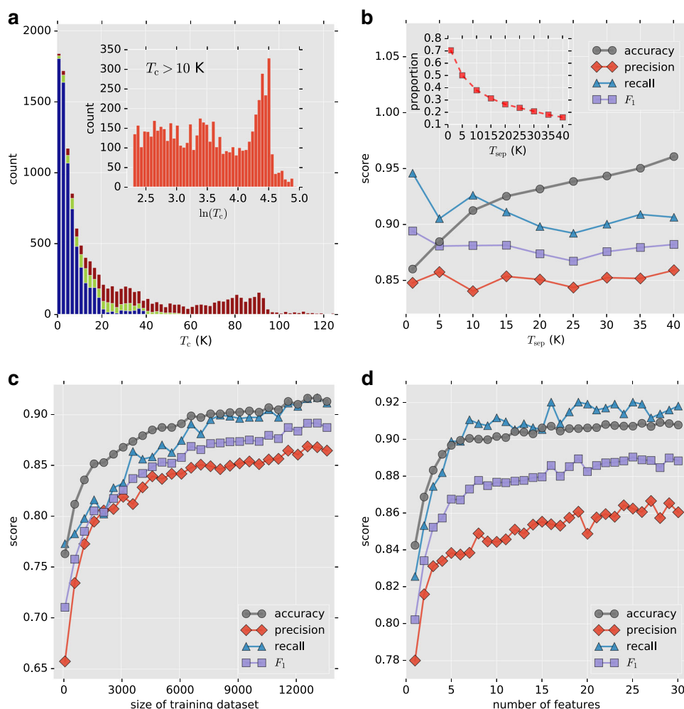
Fig. 2 SuperCon dataset and classification model performance. a Histogram of materials categorized by T_c (bin size is 2 K, only those with finite T_c are counted). Blue, green, and red denote low- T_c , iron-based, and cuprate superconductors, respectively. In the inset: histogram of materials categorized by \ln(T_c) restricted to those with T_c > 10 K. b Performance of different classification models as a function of the threshold temperature ( T_{sep} ) that separates materials in two classes by T_c . Performance is measured by accuracy (gray), precision (red), recall (blue), and F_1 score (purple). The scores are calculated from predictions on an independent test set, i.e., one separate from the dataset used to train the model. In the inset: the dashed red curve gives the proportion of materials in the above- T_{sep} set. c Accuracy, precision, recall, and F_1 score as a function of the size of the training set with a fixed test set. d Accuracy, precision, recall, and F_1 as a function of the number of predictors
